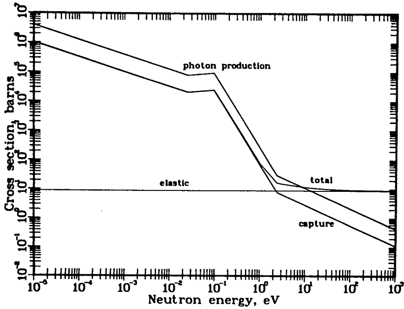
Figure 7. Slow-neutron cross sections of ^{239}\text{Pu} fission fragments.
