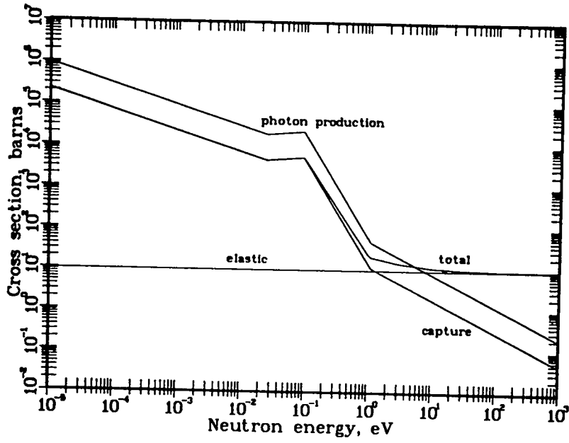
Figure 6. Slow-neutron cross sections of ^{235}\text{U} fission fragments.
