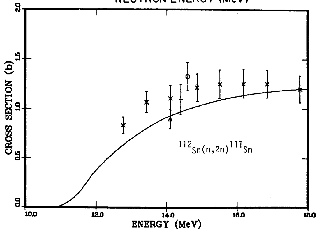
Figure 14. Comparison of calculated cross sections to experimental data for the Zr-90(n,2n) and Sn-112(n,2n) reactions.
