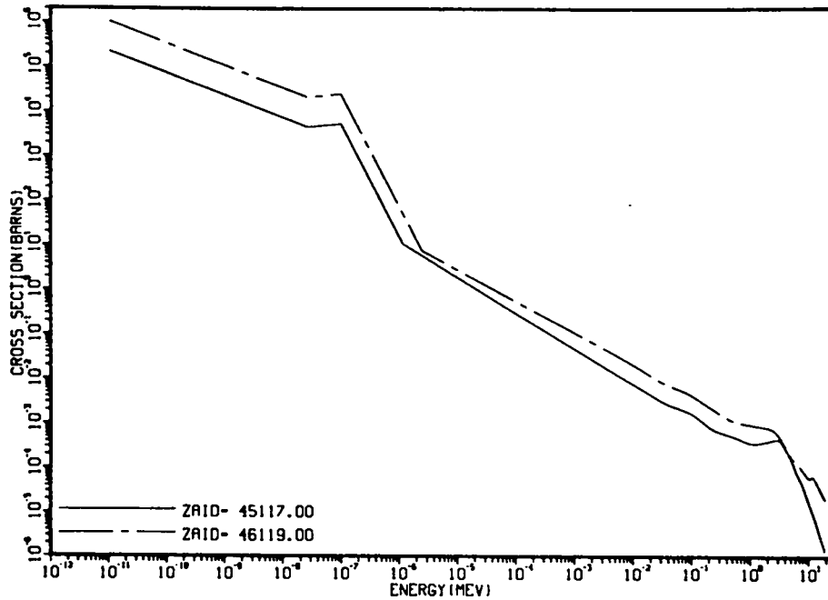
Figure 8. Comparison of the calculated capture cross sections of prompt fragments from fast fission of ^{235}\text{U} (solid line) and ^{239}\text{Pu} (broken line). The ZAI0 identifier for each case is that used in the ENDF/B version of this work and represents the average atomic and mass numbers of the respective fragments, rounded to the nearest integer.
